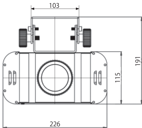
LED-WAV-50W (Versia) 寸法図
